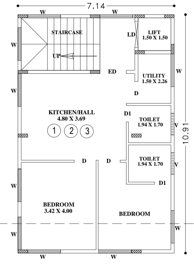
TYPICAL GROUND FLOOR 1ST & 2ND FLOOR PLAN
